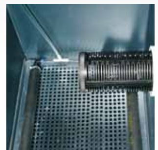
Floating Bed filter chamber
